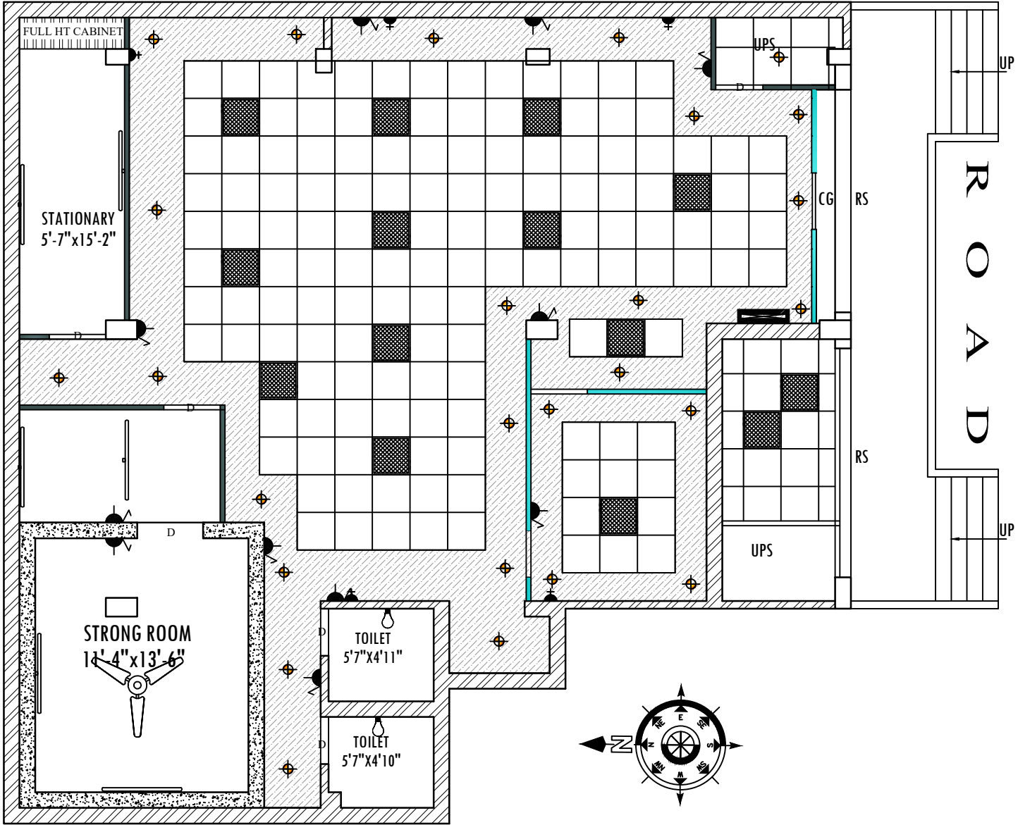
GROUND FLOOR PLAN ROOF HT :- 11'-0" BEEM HT :- 9'-6"
