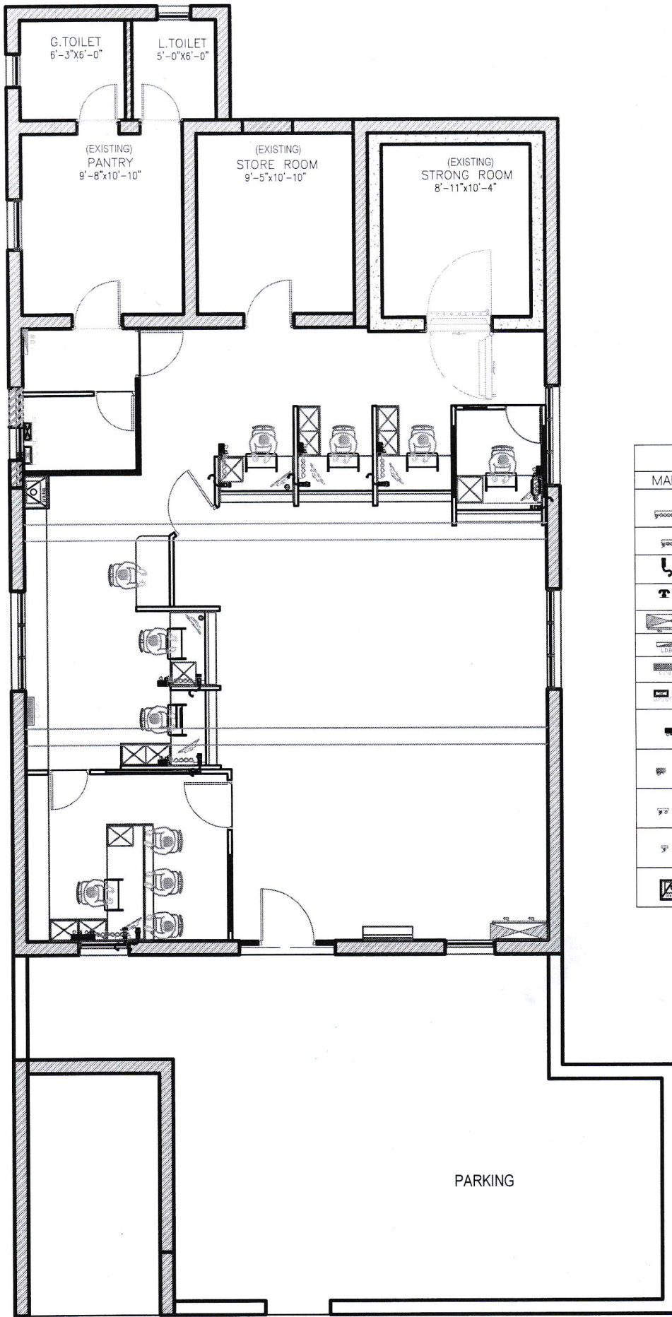
ELECTRICAL LAYOUT PLAN
