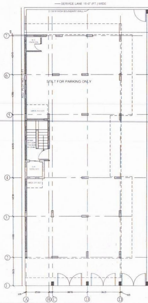
STILT PLAN
