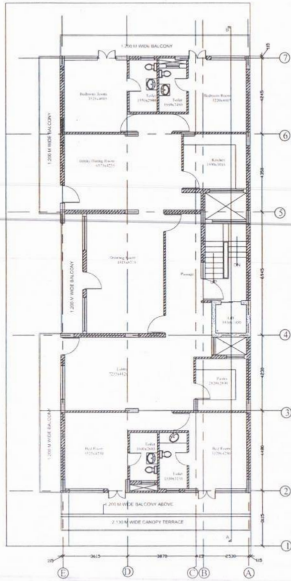
GROUND, FIRST, SECOND & THIRD FLOOR PLAN
