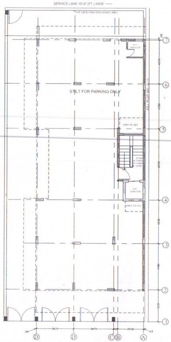
STILT PLAN
