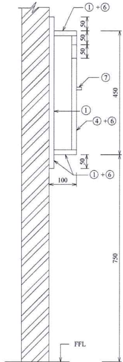
SECTION@DD
