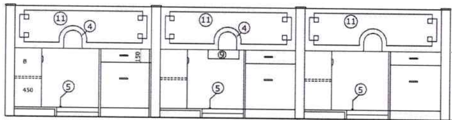
FRONT ELEVATION
