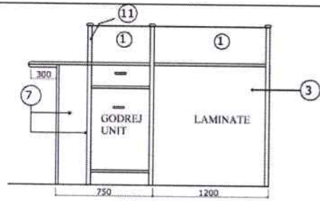
SECTION @ X
