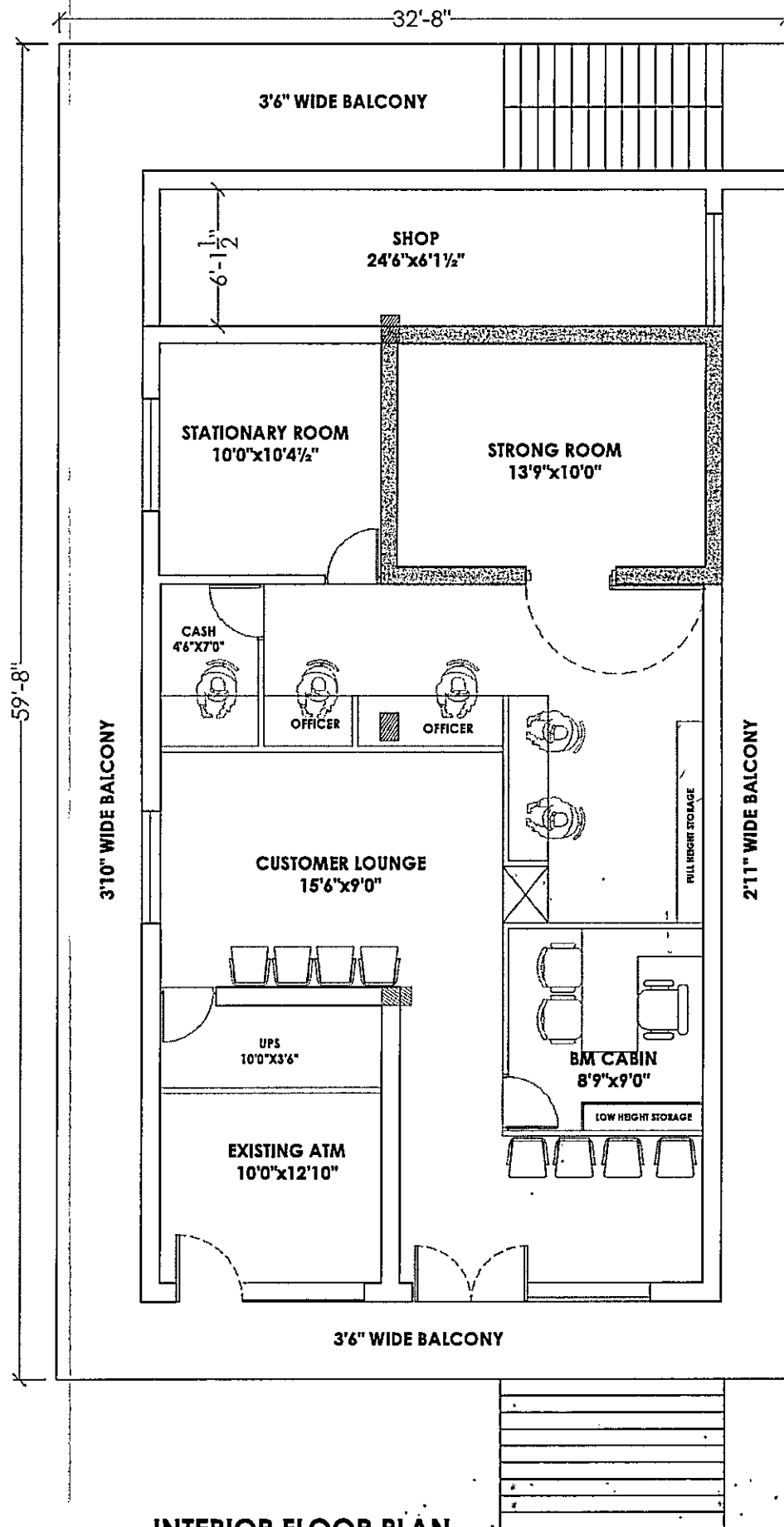
INTERIOR FLOOR PLAN
