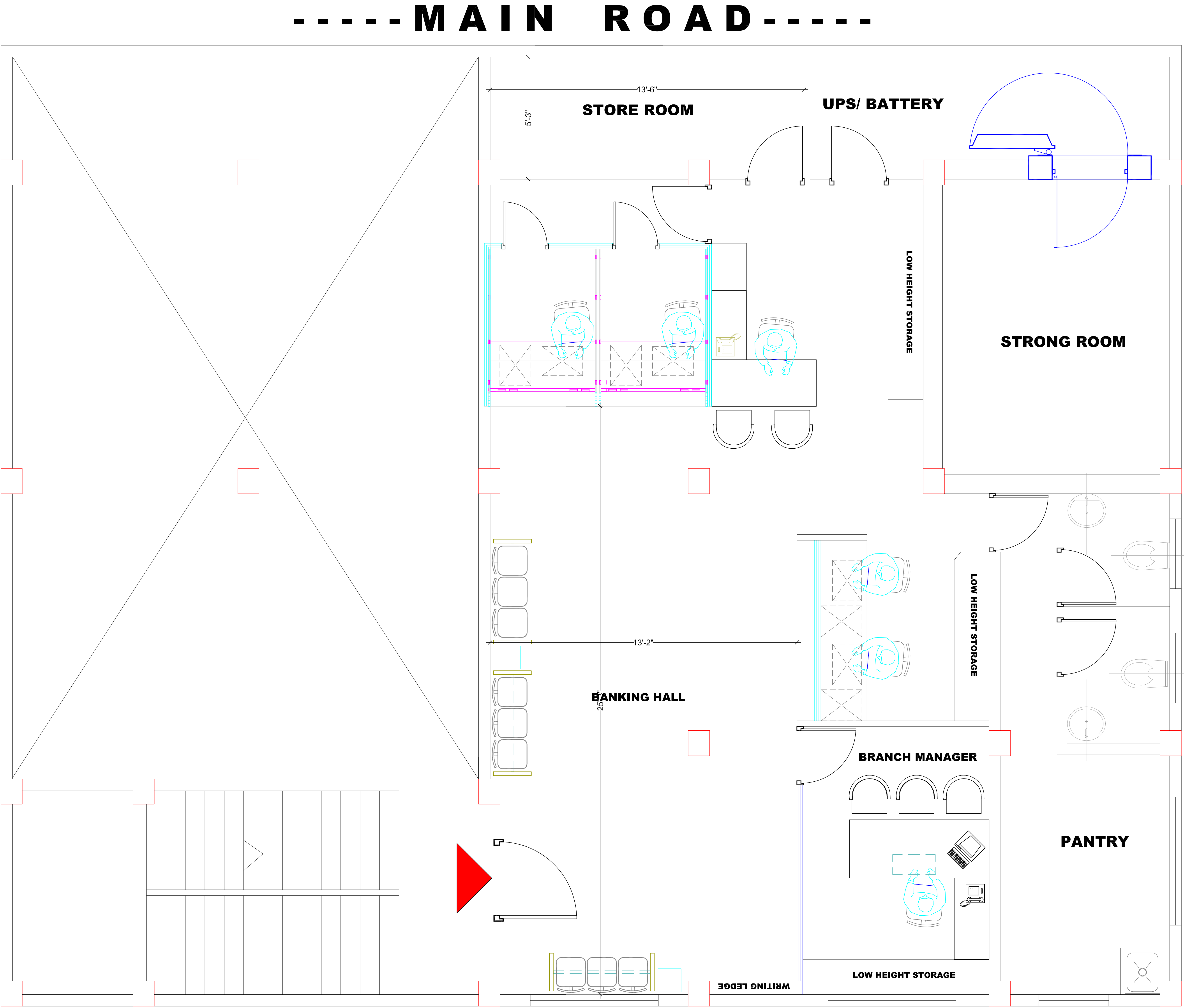
PROPOSED LAYOUT PLAN OF BIJNI BRANCH
