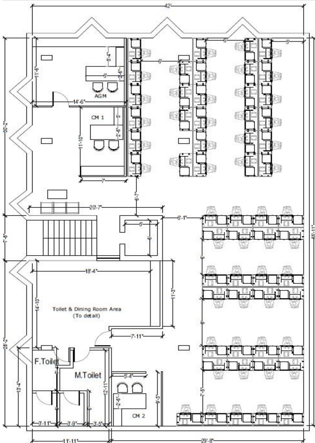
Proposed Floor plan for DAMC 2nd Floor, Kilpauk, Chennai
