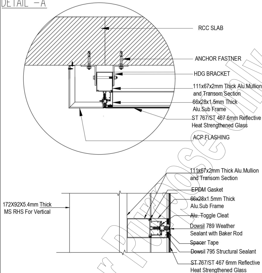
TYPICAL VERTICAL SECTION AT INTERMEDIATE HORIZONTAL SEC - A A
