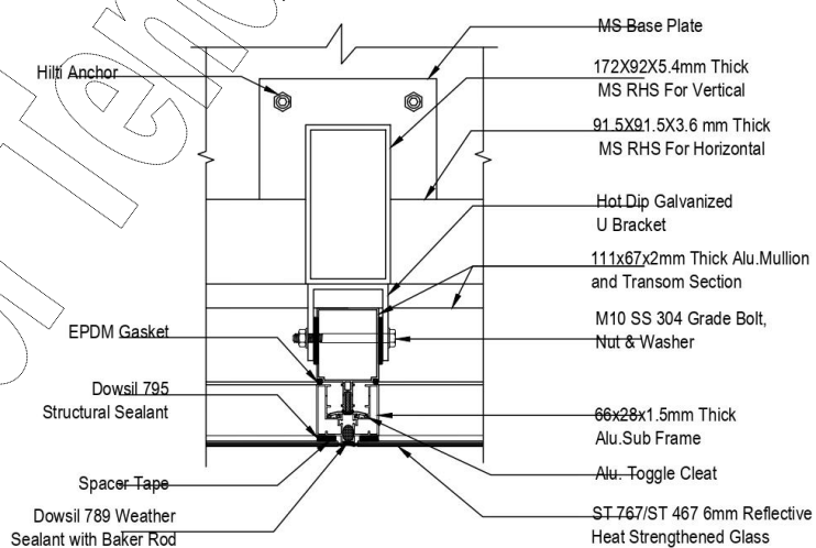
TYPICAL HORIZONTAL SECTION AT INTERMEDIATE VERTICAL SEC- B B
